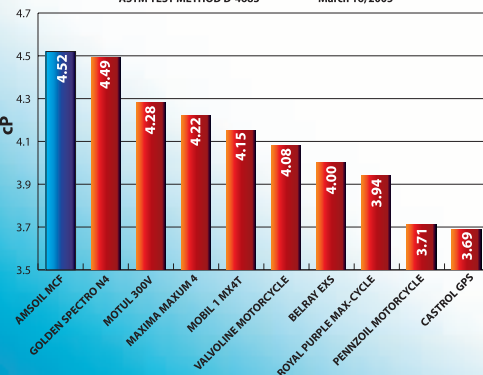
10W-40 Motorcycle Oil - High Temperature Viscosity Protection Higher values reflect better film strength. ASTM TEST METHOD D-4683 March 16, 2005
