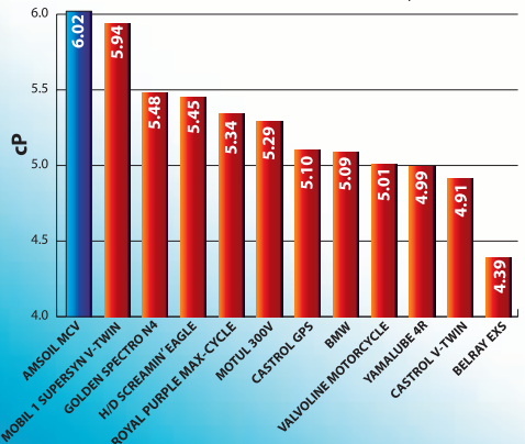
20W-50 Motorcycle Oil - High Temperature Viscosity Protection Higher values reflect better film strength. ASTM TEST METHOD D-4683 March 16, 2005
